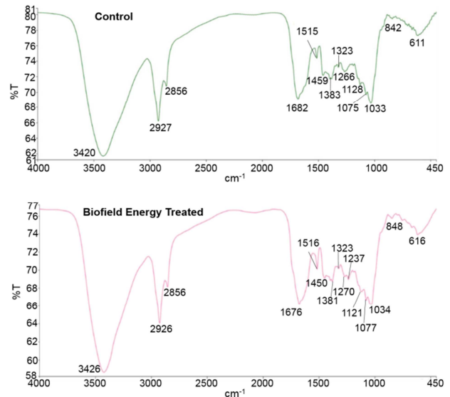
Figure 3. FT-IR spectra of the control and Biofield Energy Treated ashwagandha root extract.
